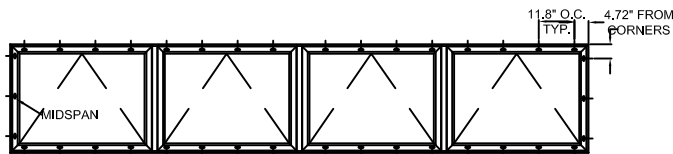
TYPICAL ELEVATION WITH FASTENER SPACING
