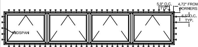
TYPICAL ELEVATION WITH FASTENER SPACING
